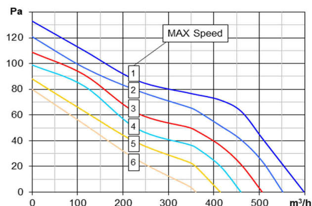
FAD(S)145N14E4.. 50Hz
