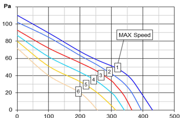
FAD(S)145M14E4.. 50Hz
