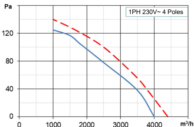
...4P540... ø400/27° — 50Hz — 60Hz
