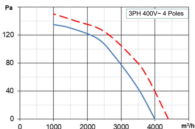
...4P540...J ø400/27° — 50Hz — 60Hz
