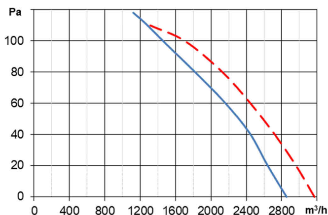
ER4L535S. ø350/27° — 50Hz — 60Hz
