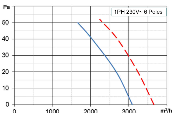
...6P540... ø400/33° — 50Hz — 60Hz
