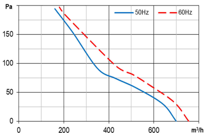
ER2L2 / C2L2 / L22 Ø172/31°
