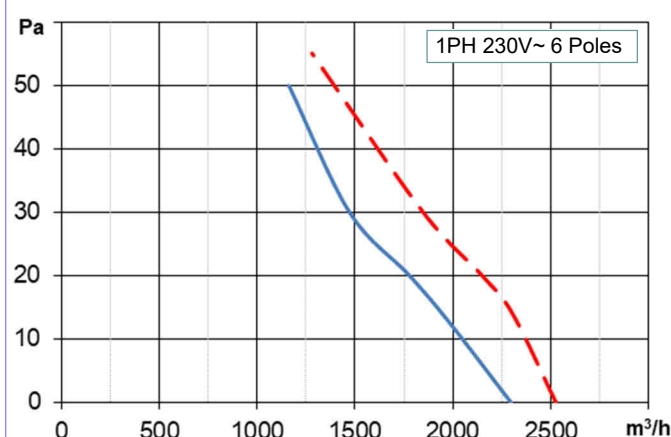
...6P335... ø350/33° — 50Hz — 60Hz
