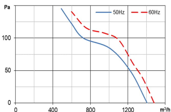
ER2L3 / C2L3 / L23 Ø230/27°
