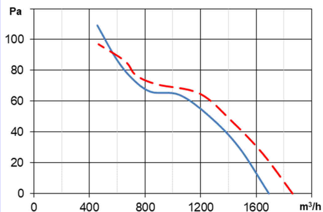
ER4L330S. ø 300/27° — 50Hz — 60Hz
