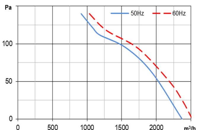
ER2L5 / C2L5 / L25 Ø300/16°
